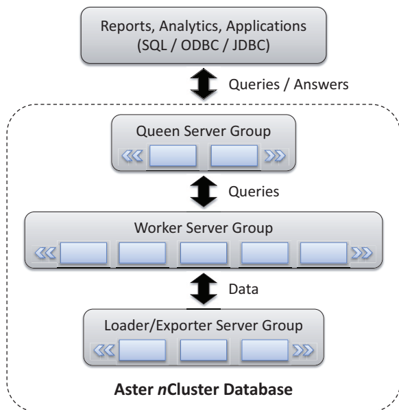
Figure 5: nCluster Architecture
